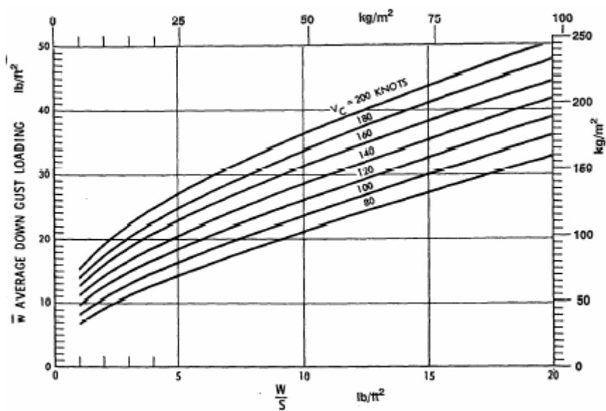
FIGURE B3 UP AND DOWN GUST LOADING ON HORIZONTAL TAIL SURFACE.
