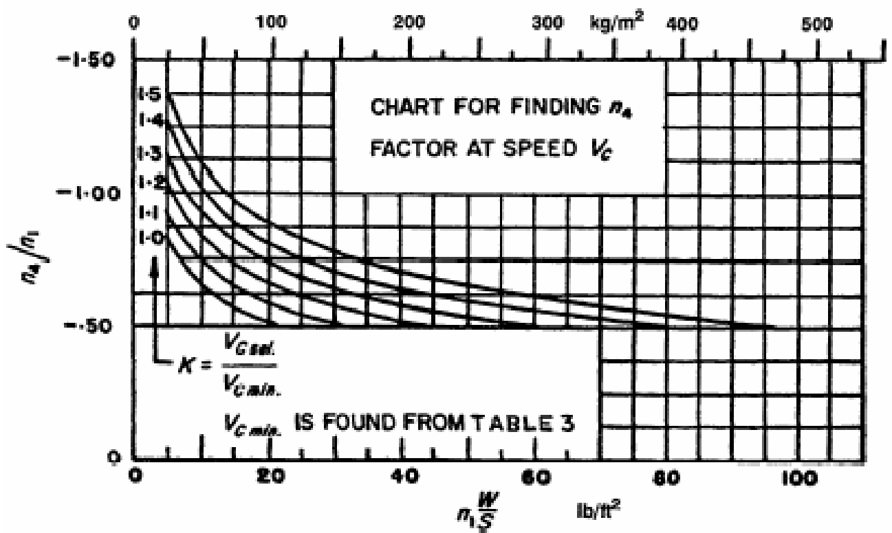
FIGURE A2 CHART FOR FINDING n_4 FACTOR AT SPEED V_c .
