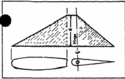
FIGURE B7 TAIL SURFACE LOAD DISTRIBUTION.
