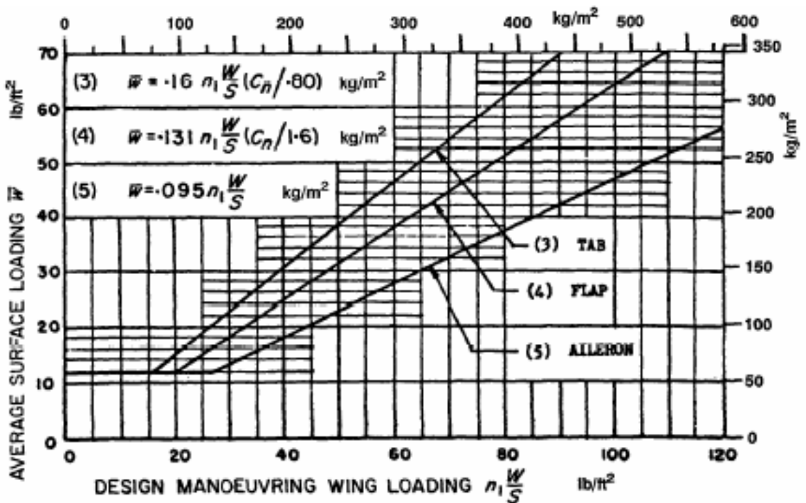
FIGURE A5 AVERAGE LIMIT CONTROL SURFACE LOADING.
