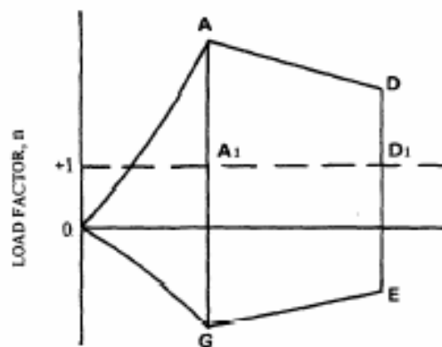
FIGURE 1 PITCHING MANOEUVRES
