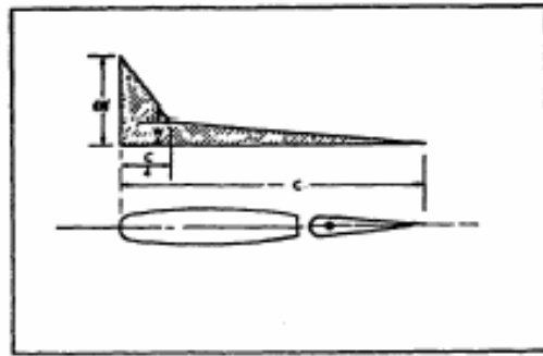
FIGURE B8 TAIL SURFACE LOAD DISTRIBUTION.
