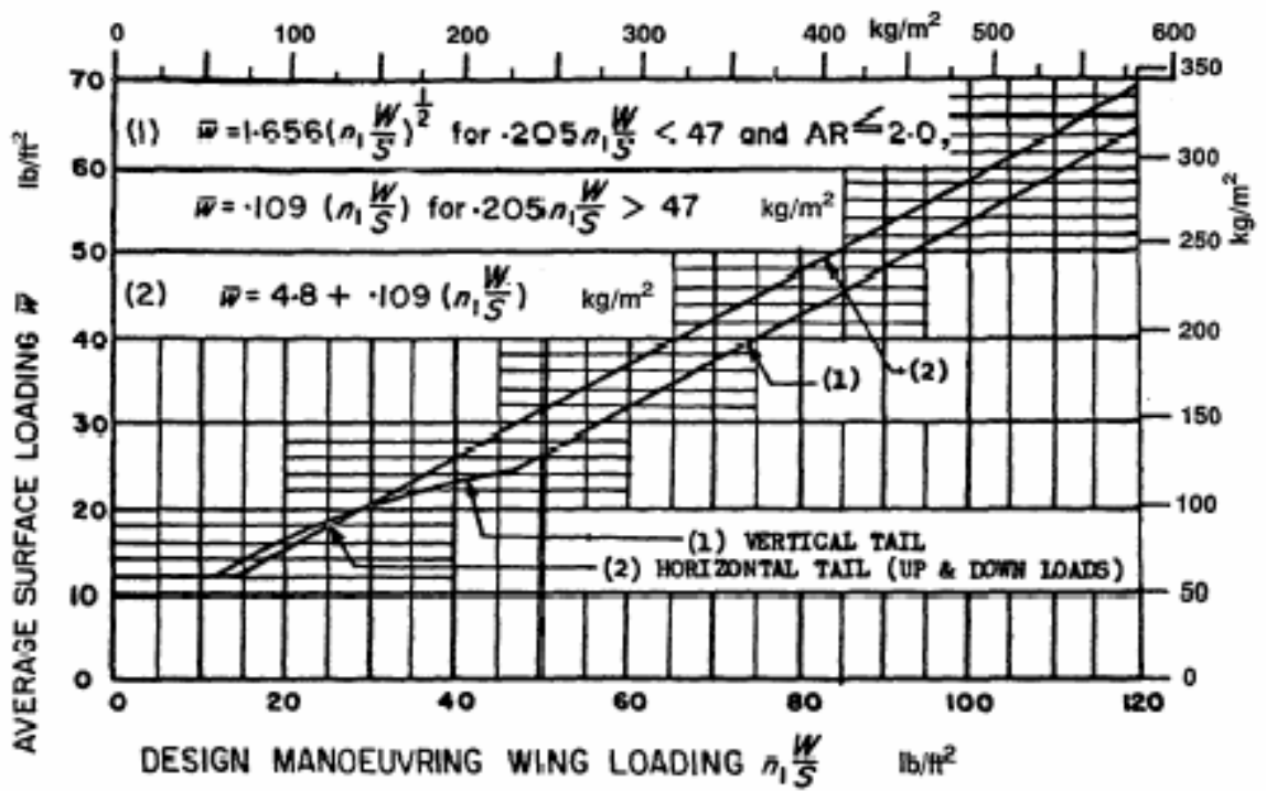
FIGURE A4 AVERAGE LIMIT CONTROL SURFACE LOADING.
