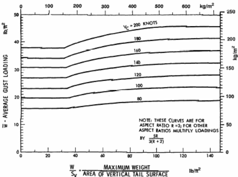
FIGURE B5 - GUST LOADING ON VERTICAL TAL SURFACE.
