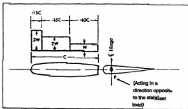
FIGURE B6 - TAIL SURFACE LOAD DISTRIBUTION.
