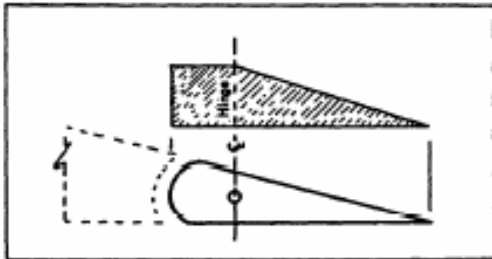
FIGURE B9 AILERON LOAD DISTRIBUTION.
